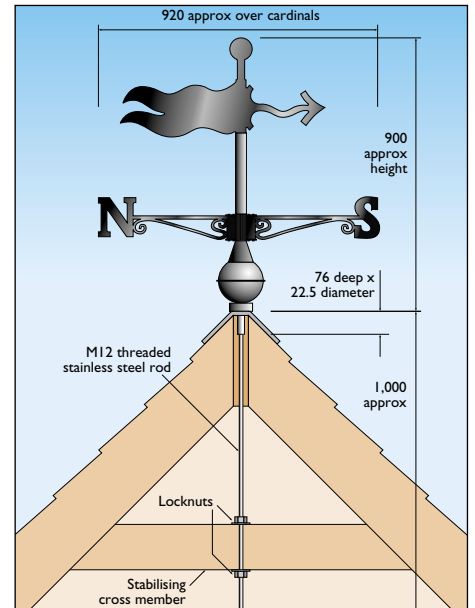
Dimensions and installation method for medium windvanes
