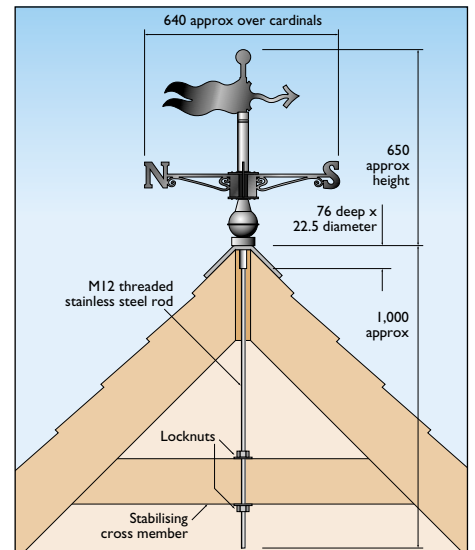
Dimensions and installation method for small windvanes
