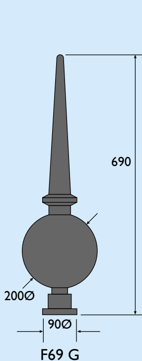
Standard finial range
