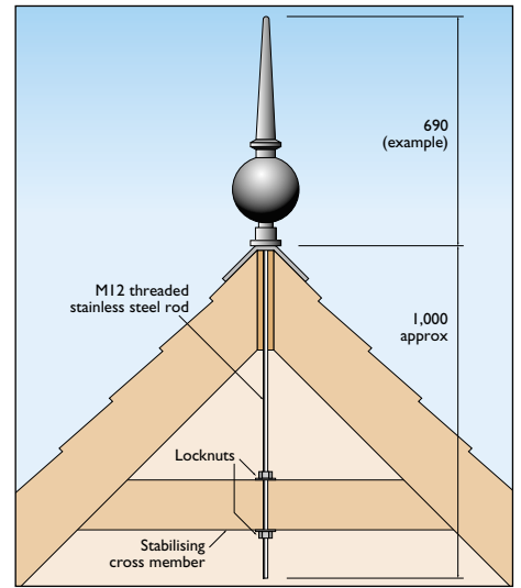
Installation method (F69 shown)
