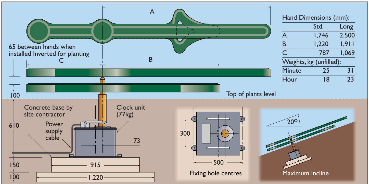
Overall dimensions, weights and installation details
